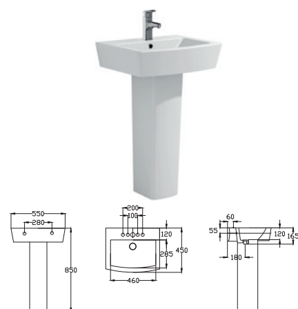
Washbasin with pedestal VS-WB180-A 550 x 450 x 850mm
