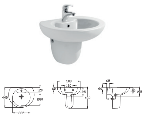
Washbasin with half pedestal VS-WB300-B 450 x 395 x 460mm 500 x 440 x 460mm
