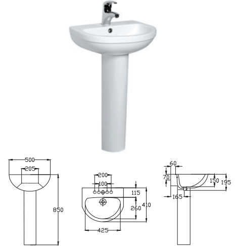
Washbasin with pedestal VS-WB230-A 500 x 410 x 850mm
